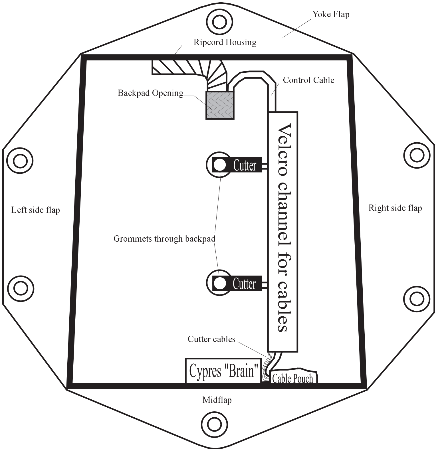
Figure 1: Elite series reserve pack tray layout
